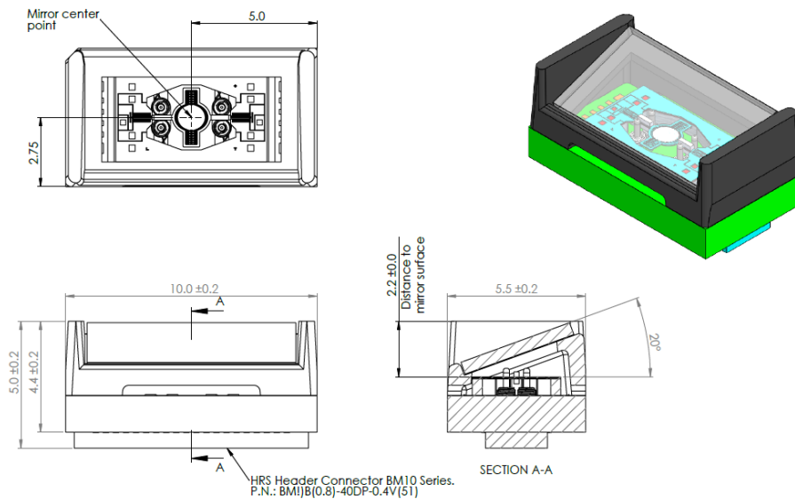
Figure 2: Scanning Head Module General View
