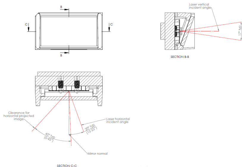
Figure 3: Scanning Head Module General View
